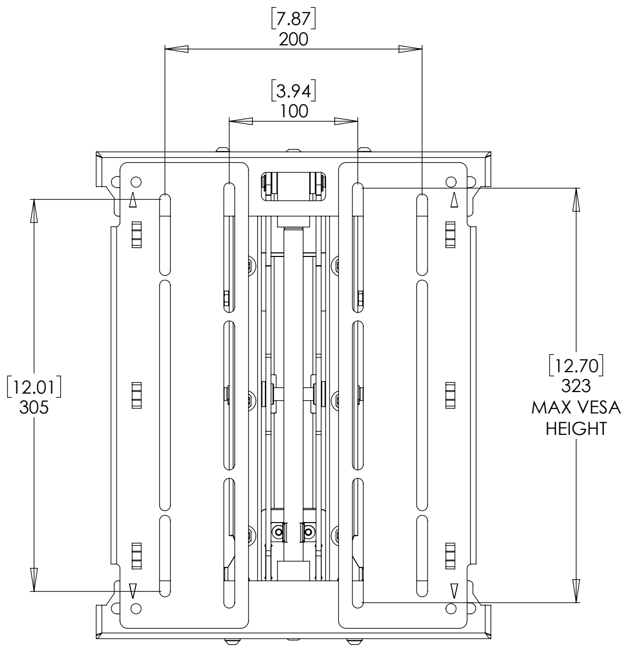
DEFAULT MOUNT ORIENTATION
