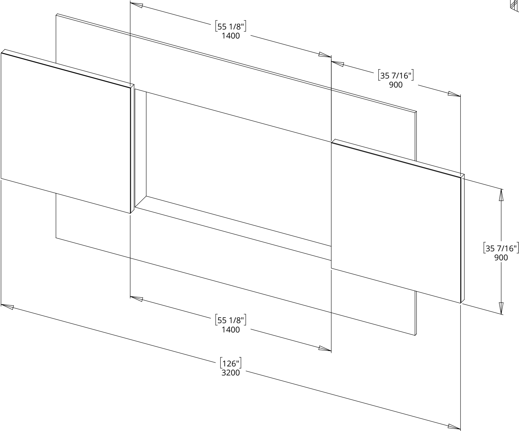
DETAIL B
